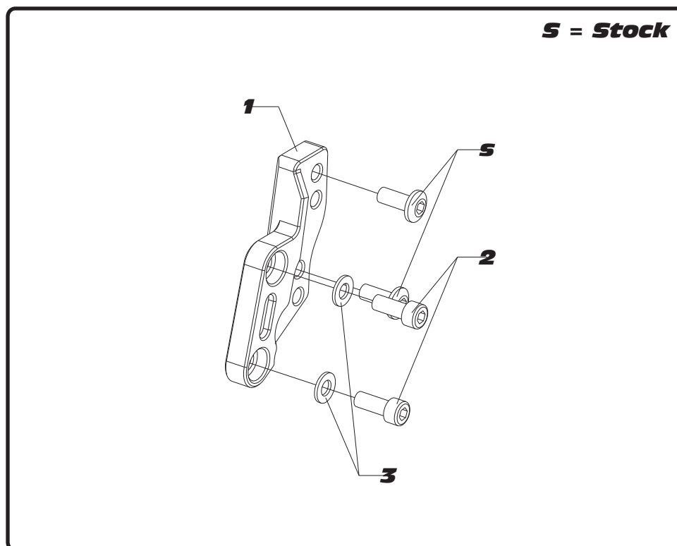
Parts Diagram
