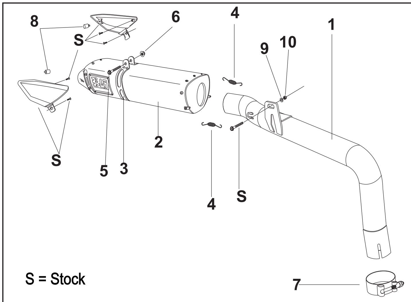
Parts Diagram
