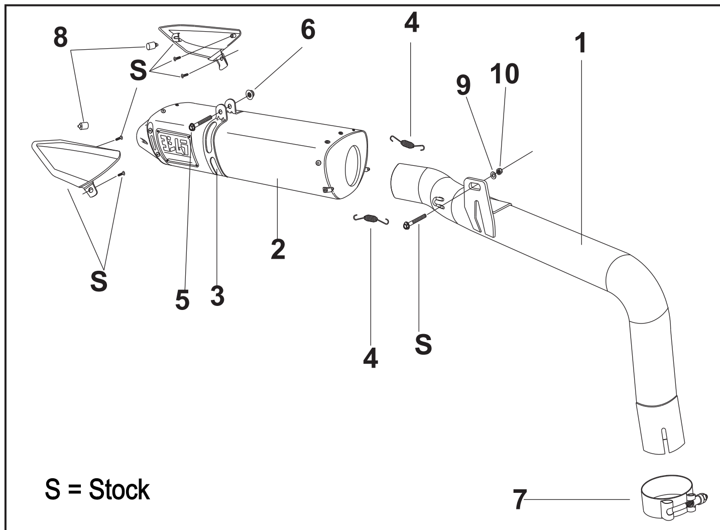
Parts Diagram
